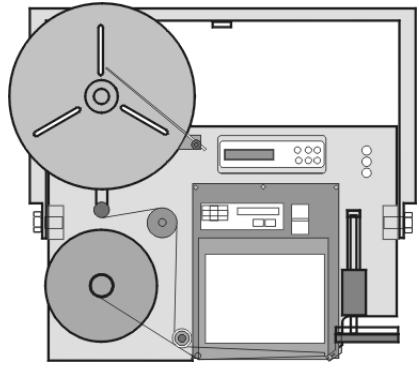
250 Printer Applicator
