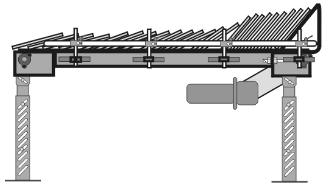
Optional Shingling Conveyor
